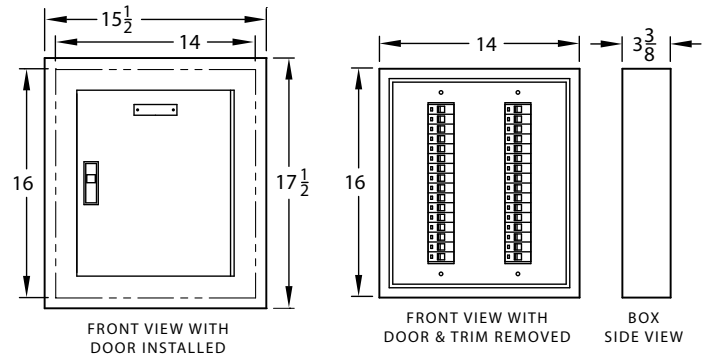
Flush Trim Panel - up to 32 Circuits
